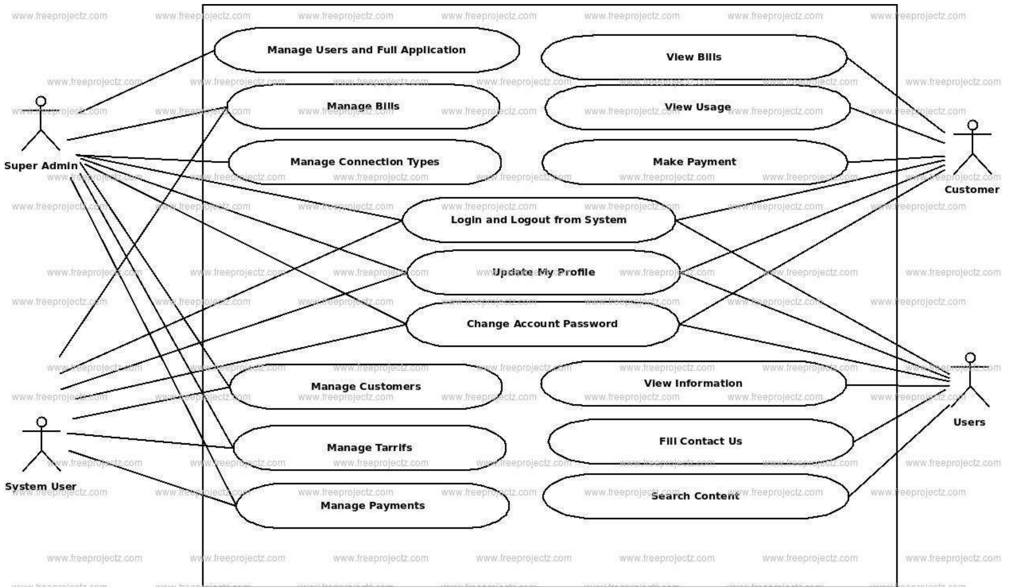
Usecase Diagram of Telephone Billing Payment System
