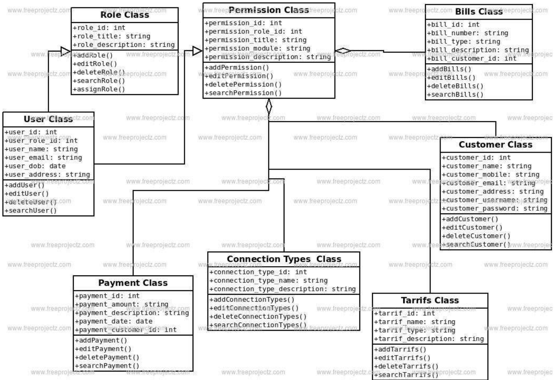
Class Diagram of Mobile Phone Billing System
